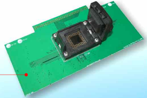
BGA adapter 456 pins, 1.00mm pitch
