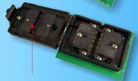
Universal SOIC adapter One adapter to test devices up to 44 pins with body widths from 0.150" to 0.6"
